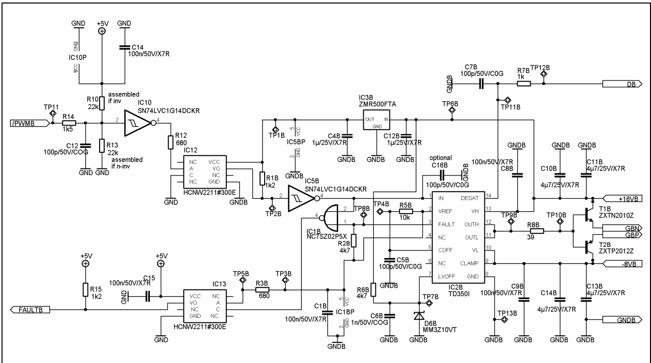
Figure 11 IGBT driver – Bottom transistor
