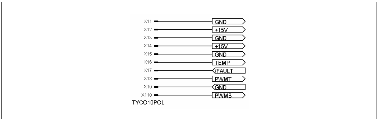
Figure 16 IGBT driver – External connections
