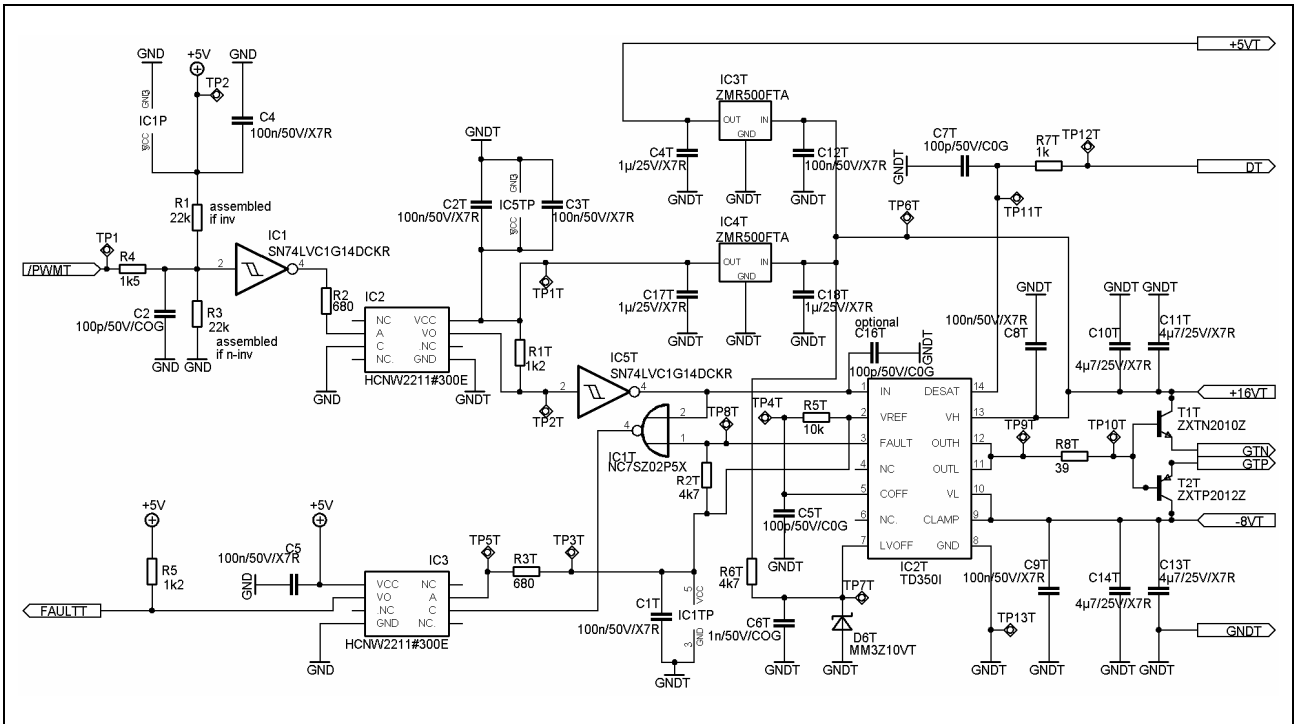
Figure 10 IGBT driver – Top transistor
