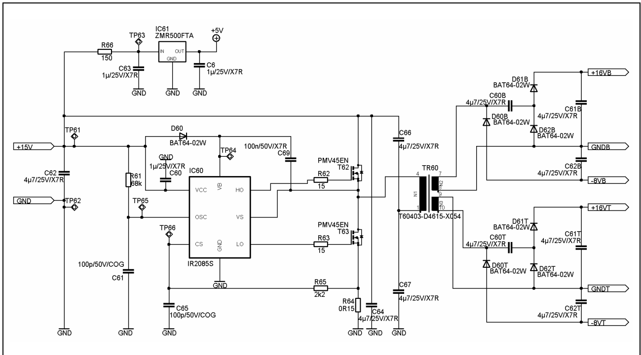
Figure 15 IGBT driver – DC/DC converter
