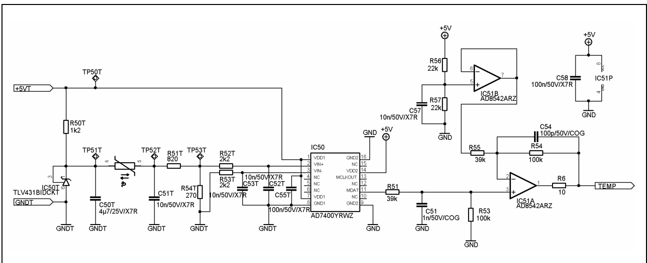
Figure 14 IGBT driver – Temperature measurement
