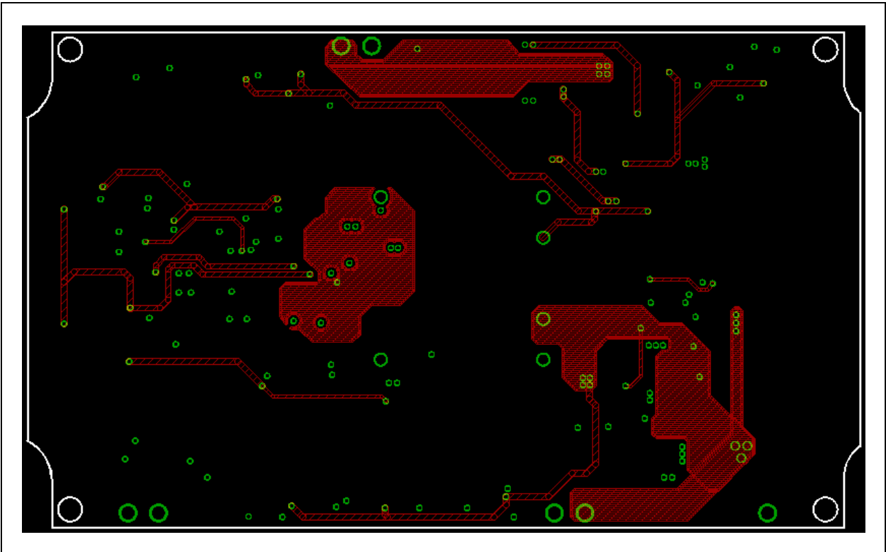
Figure 19 IGBT driver – Layer 3
