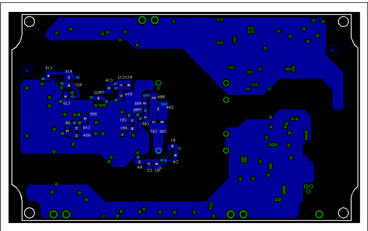
Figure 20 IGBT driver – Layer 4 (Bottom)
