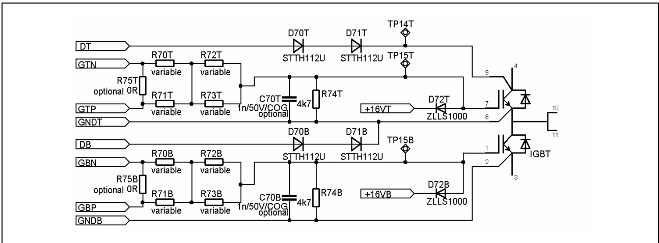
Figure 12 IGBT driver – Module connectors
