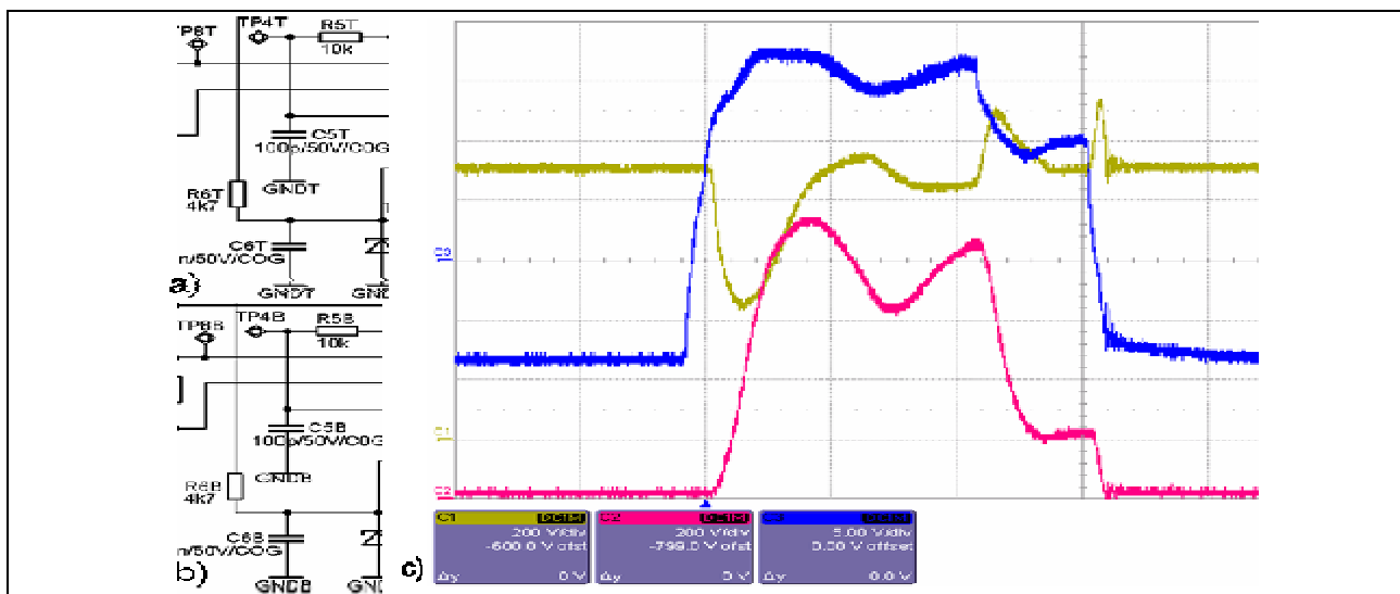
Figure 6 a, b) 2-level Turn-off circuit with values to be adjusted if L_{\sigma} > 30\text{nH} , c) switching-off under short circuit conditions
