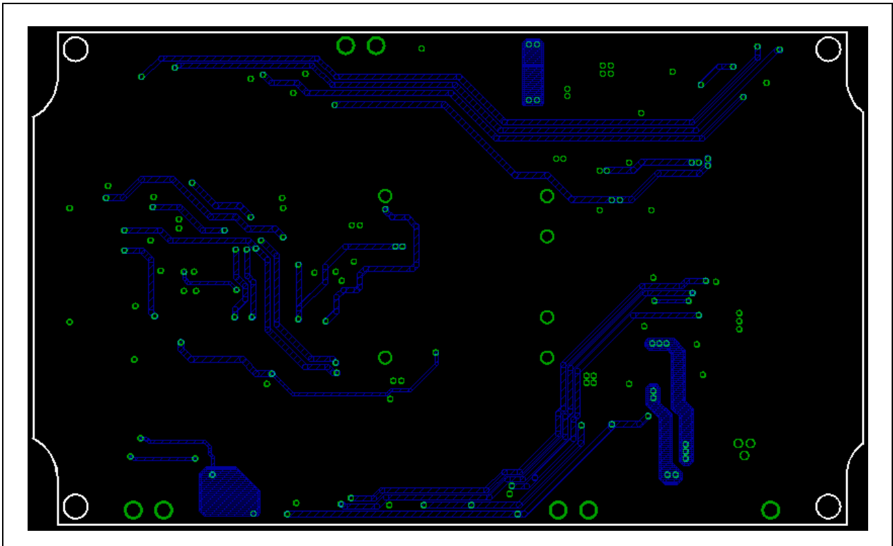
Figure 18 IGBT driver – Layer 2
