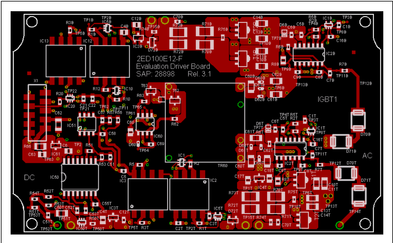
Figure 17 IGBT driver – Layer 1 (Top)
