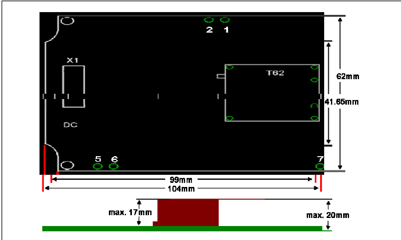
Figure 3 Dimensions of the 2ED100E12-F
