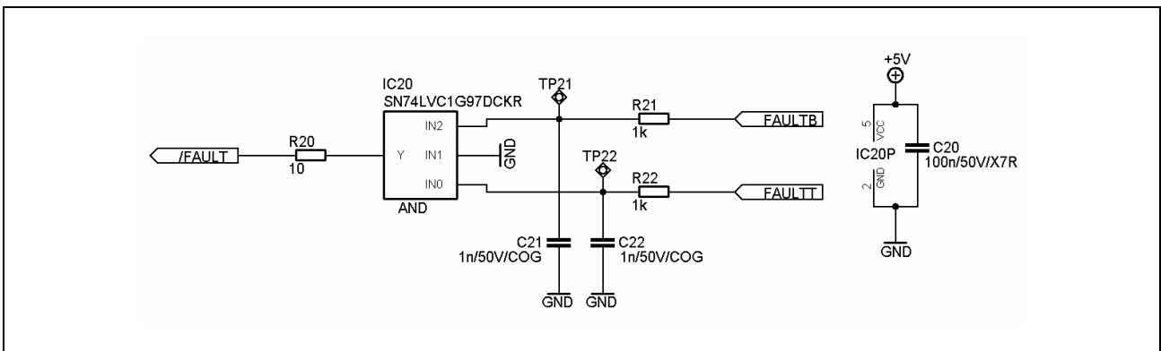
Figure 13 IGBT driver – Fault output
