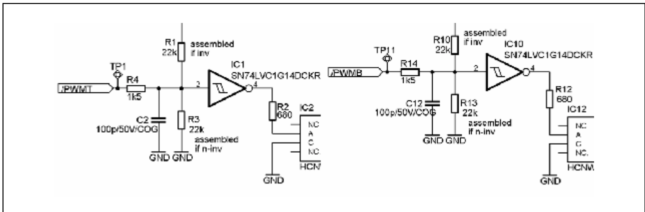
Figure 4 Schematic of the input circuit.
