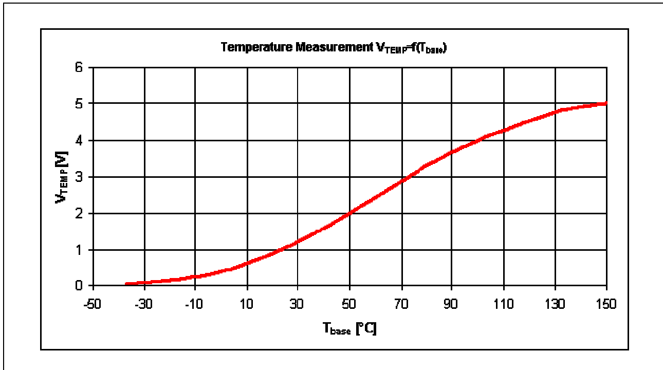
Figure 9 Characteristic of the temperature measurement
